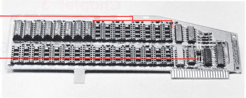
Figure 3-1 512K upgrade
