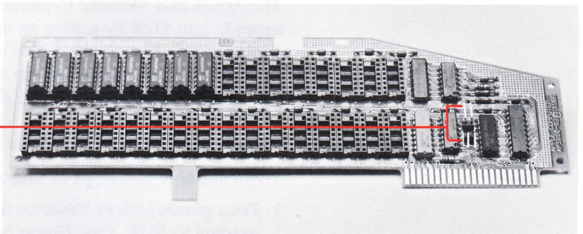
Figure 3-2 1-megabyte upgrade
